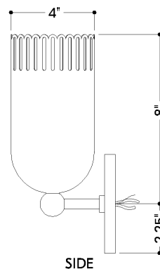
SIDE
